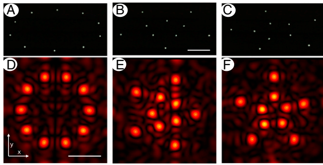
Fig. 2. Simultaneous in-plane manipulation of 10 EPS particles of 2-mm diameter. The particles are trapped 2.3 mm ( \lambda/4 ) above a reflective surface. (A) The particles start in a circle, (B) odd particles move toward the center, and (C) the two concentric circles of particles rotate in opposite directions. (D–F) The simulated pressure-amplitude fields generated at the reflective surface. The 16 \times 16 array was placed parallel to the surface 13 cm above it. (Scale bar, B and D: 2 cm.)
